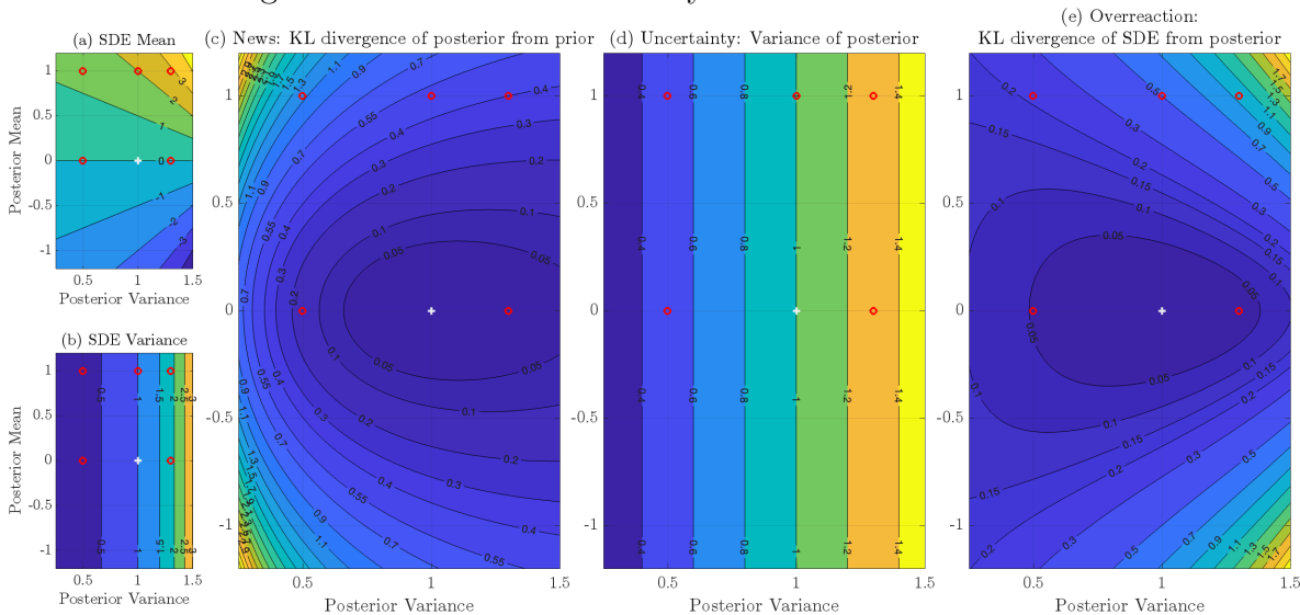
Figure 6: News and uncertainty in a Normal distribution
